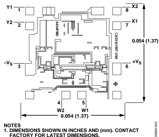
Figure 2. Metallization Photograph
